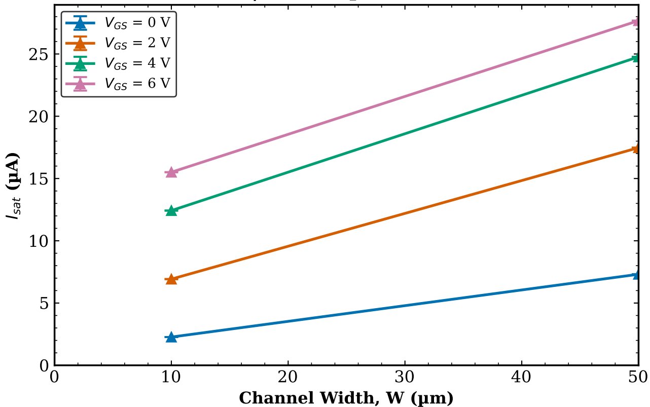
TFT2 Transistor 1 I_{sat} vs W | L = 20\text{ }\mu\text{m} (mean \pm std)
